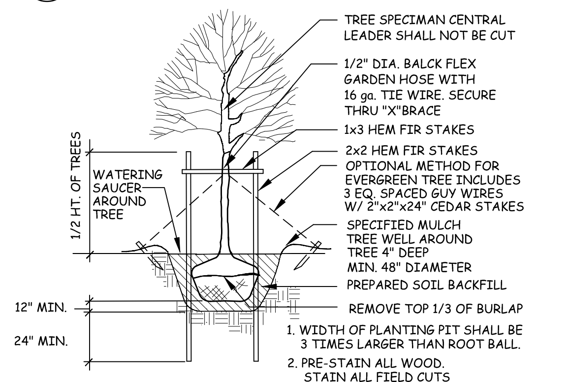
4 TYPICAL DECIDUOUS TREE PLANTING SCALE: N.T.S.
